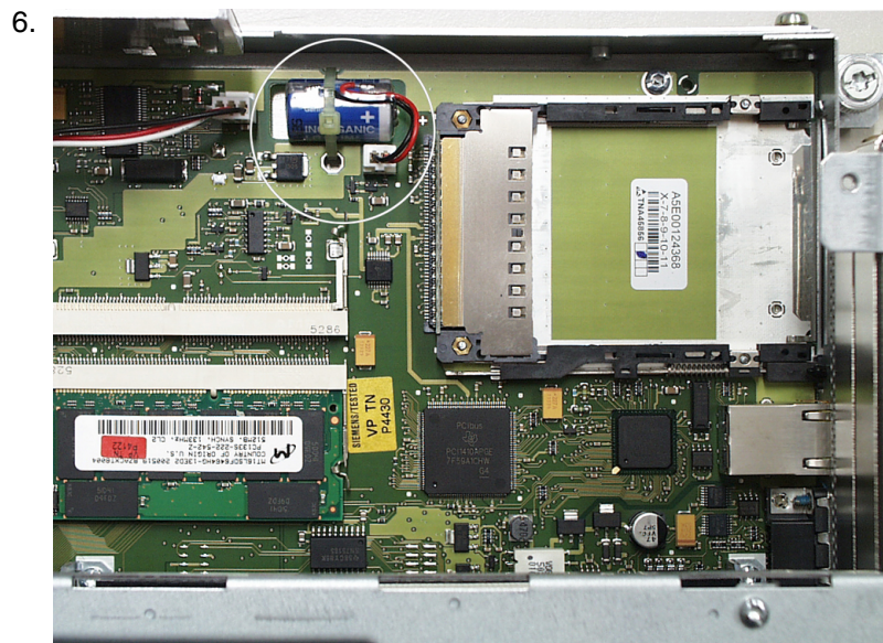
Example: PCU50.1 and PCU50.2 battery replacement
